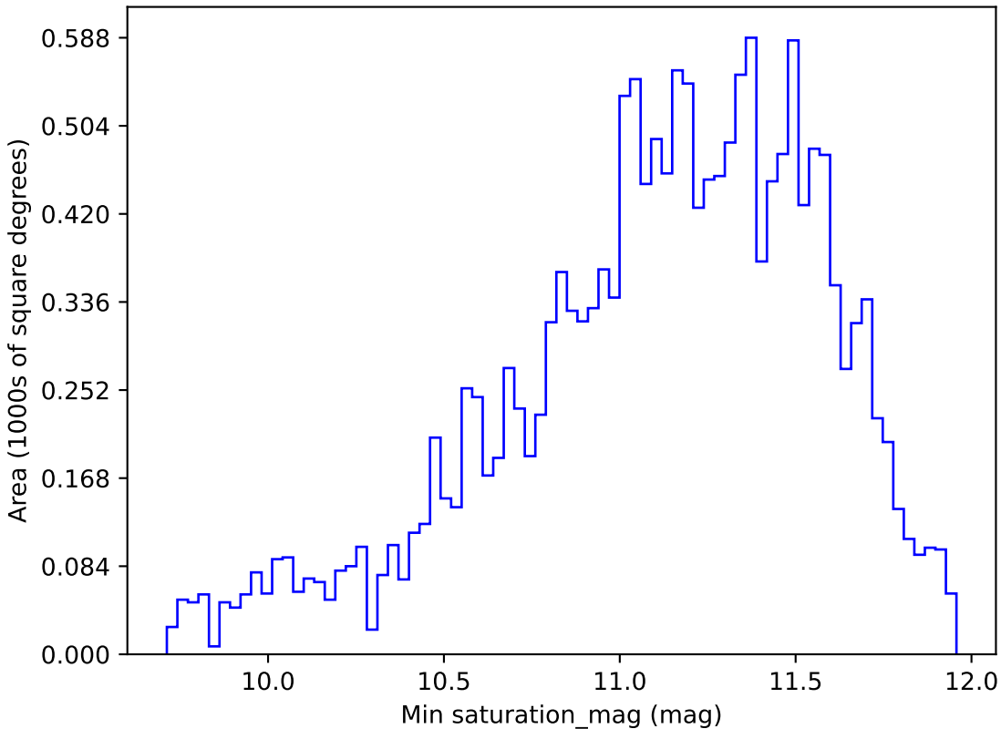
noroll_mjdp120_v3.4_10yrs WFD all bands: Min saturation_mag
