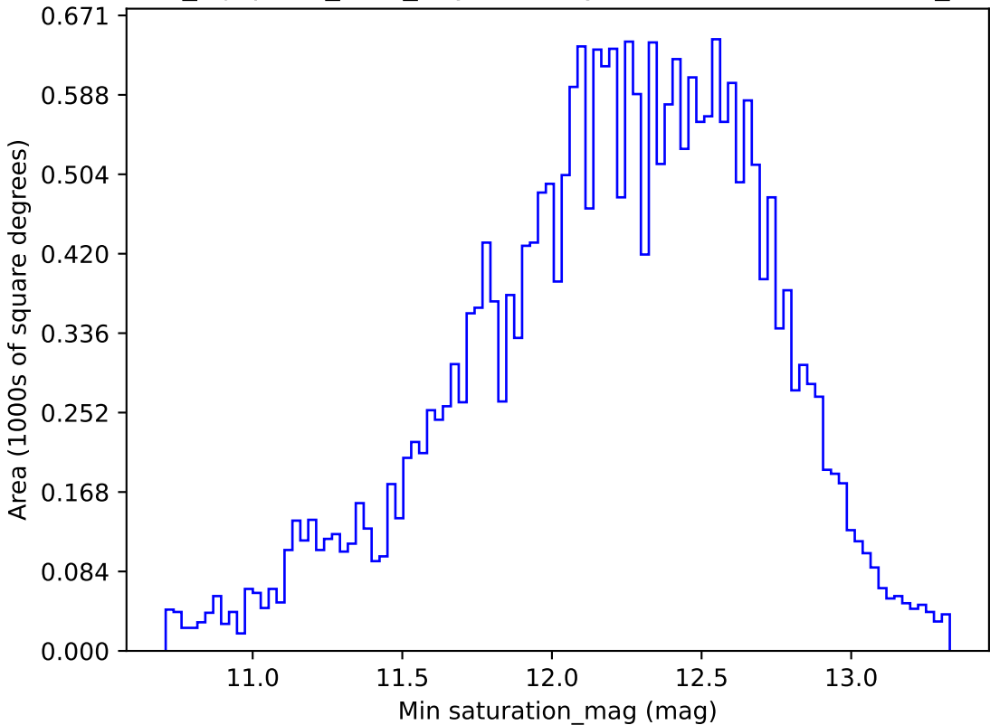
noroll_mjdp120_v3.4_10yrs All sky z band: Min saturation_mag
