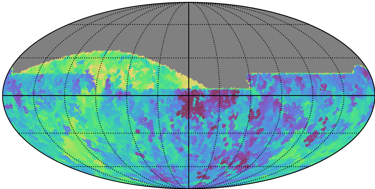
noroll_mjdp120_v3.4_10yrs All sky all bands: Min saturation_mag
