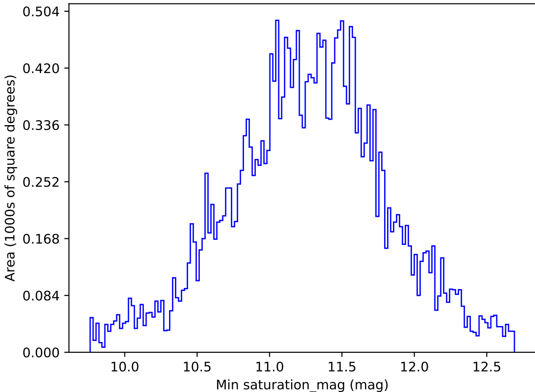
noroll_mjdp120_v3.4_10yrs All sky all bands: Min saturation_mag
