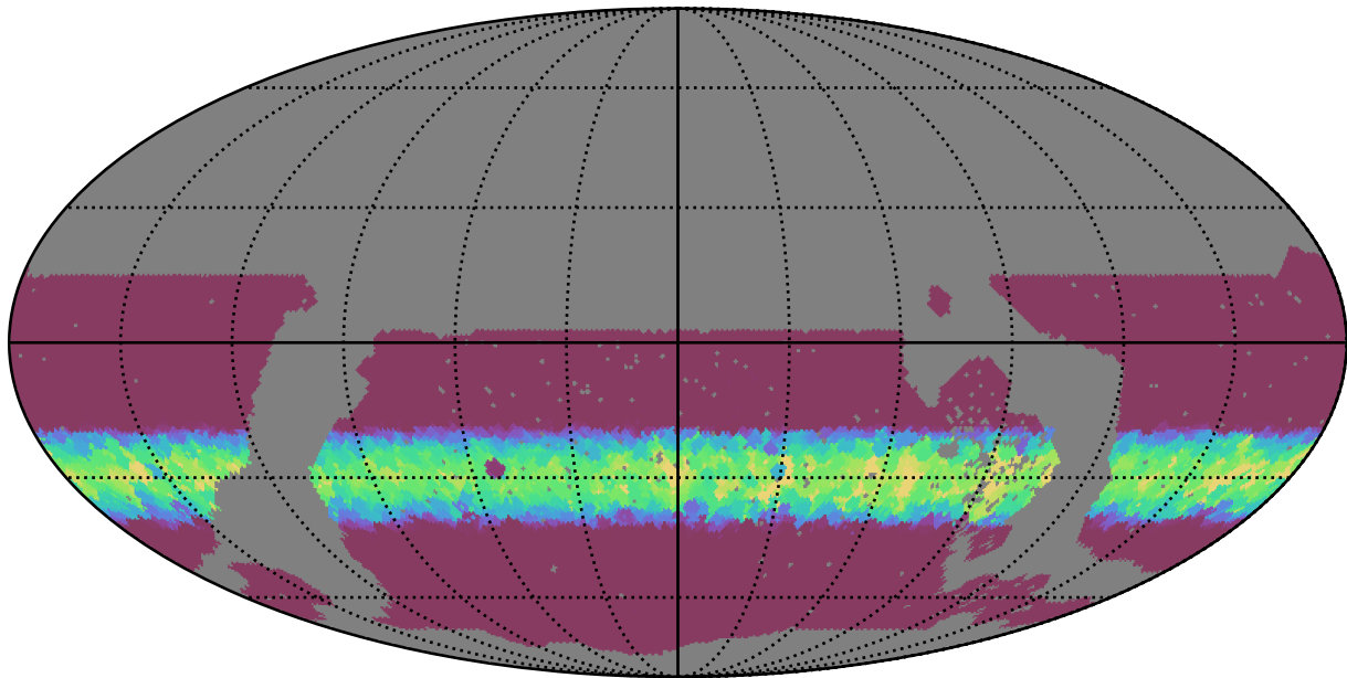
noroll_mjdp120_v3.4_10yrs WFD z band: Min normairmass
