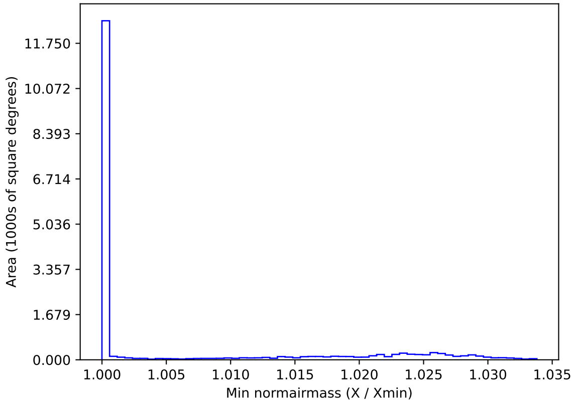
noroll_mjdp120_v3.4_10yrs WFD z band: Min normairmass
