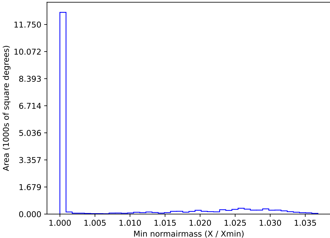
noroll_mjdp120_v3.4_10yrs WFD y band: Min normairmass
