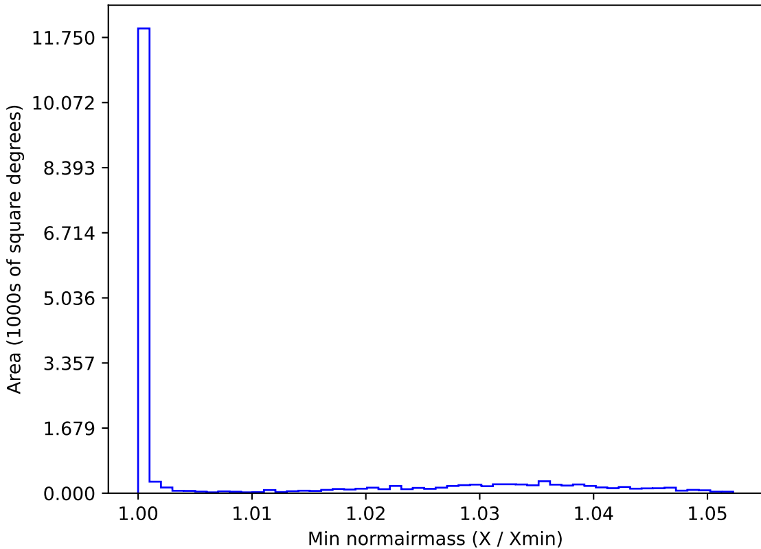
noroll_mjdp120_v3.4_10yrs WFD u band: Min normairmass
