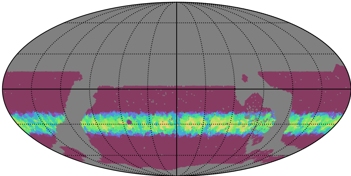
noroll_mjdp120_v3.4_10yrs WFD r band: Min normairmass
