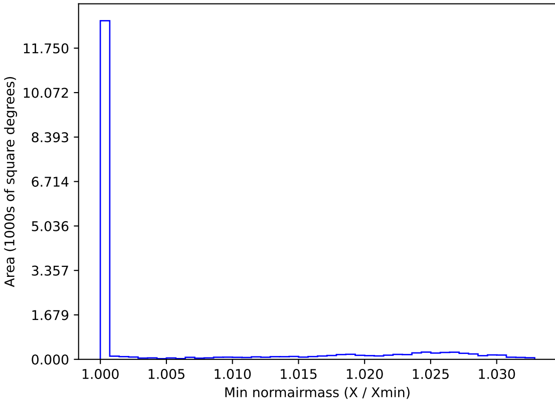
noroll_mjdp120_v3.4_10yrs WFD i band: Min normairmass
