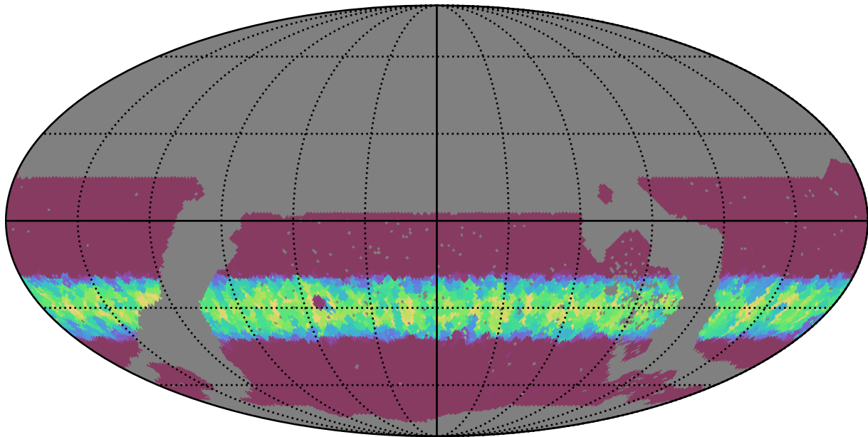
noroll_mjdp120_v3.4_10yrs WFD g band: Min normairmass
