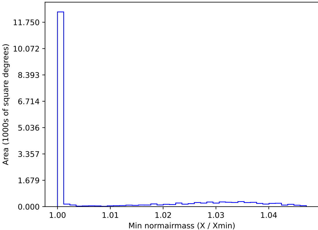
noroll_mjdp120_v3.4_10yrs WFD g band: Min normairmass
