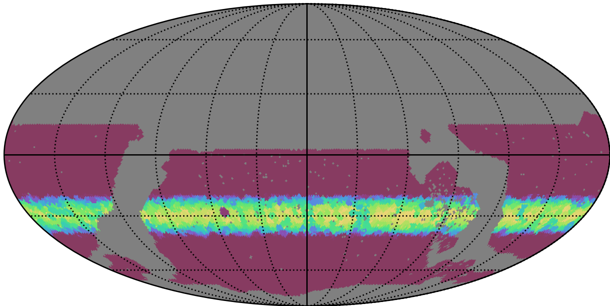
noroll_mjdp120_v3.4_10yrs WFD all bands: Min normairmass
