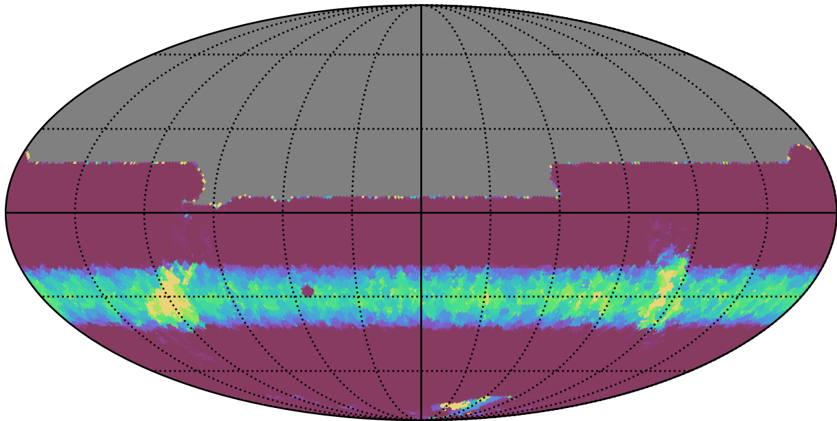
noroll_mjdp120_v3.4_10yrs All sky y band: Min normairmass
