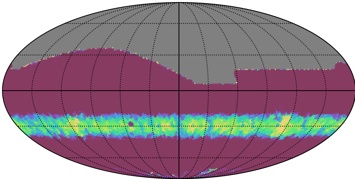
noroll_mjdp120_v3.4_10yrs All sky r band: Min normairmass
