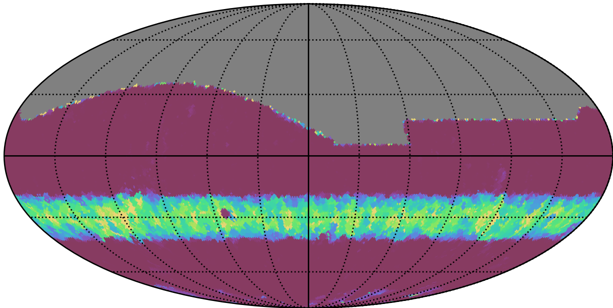
noroll_mjdp120_v3.4_10yrs All sky g band: Min normairmass
