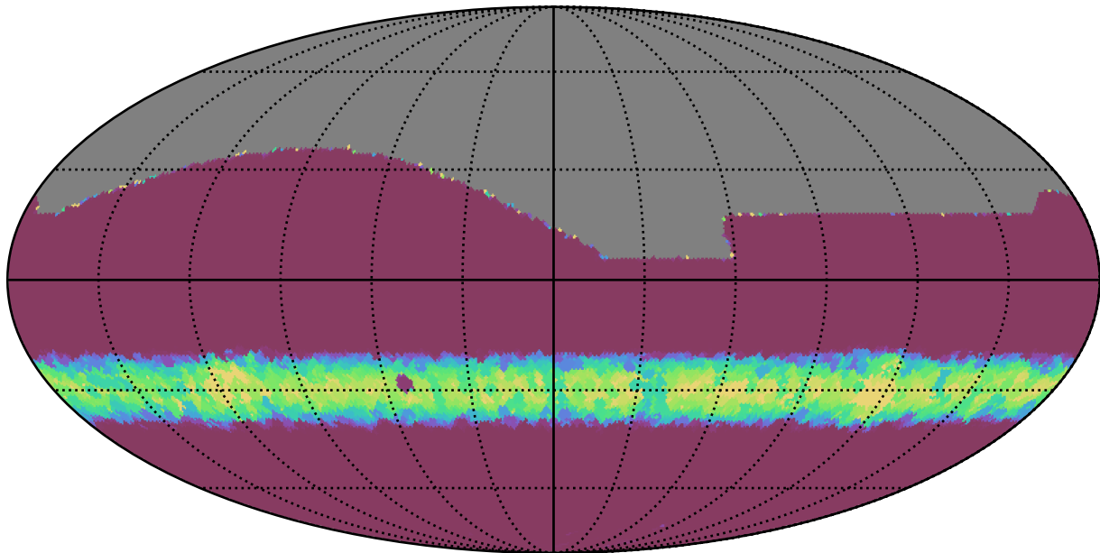
noroll_mjdp120_v3.4_10yrs All sky all bands: Min normairmass
