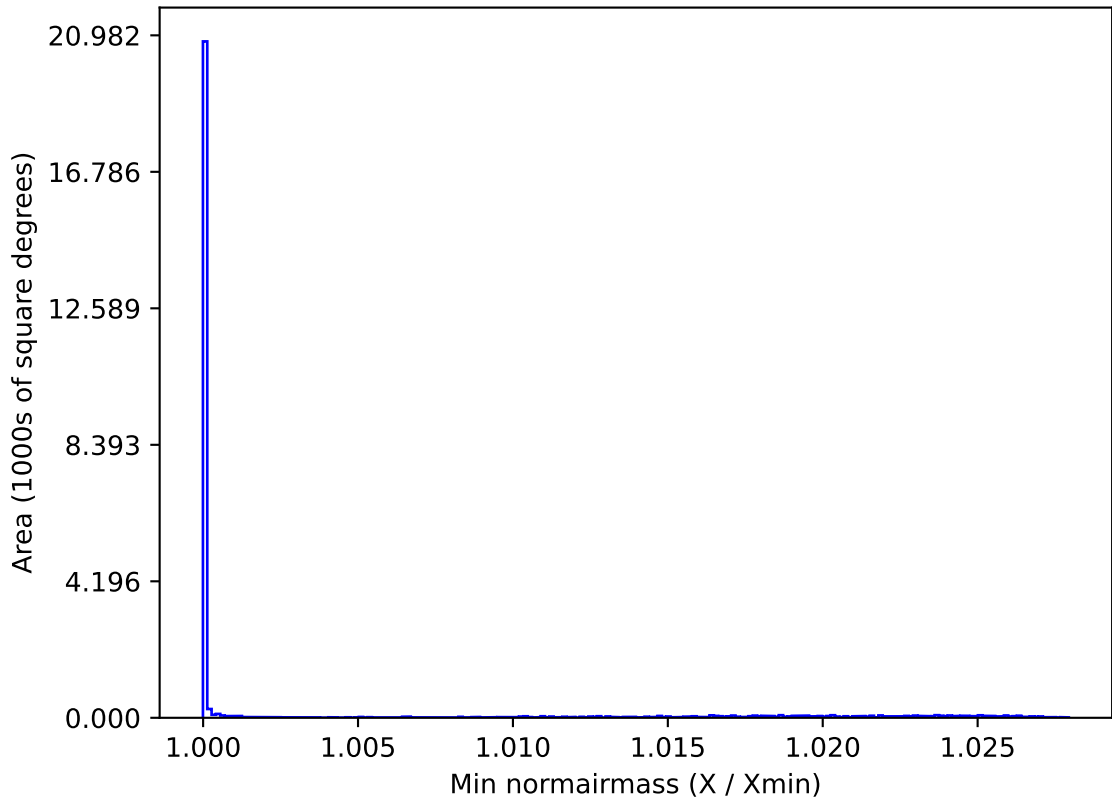
noroll_mjdp120_v3.4_10yrs All sky all bands: Min normairmass
