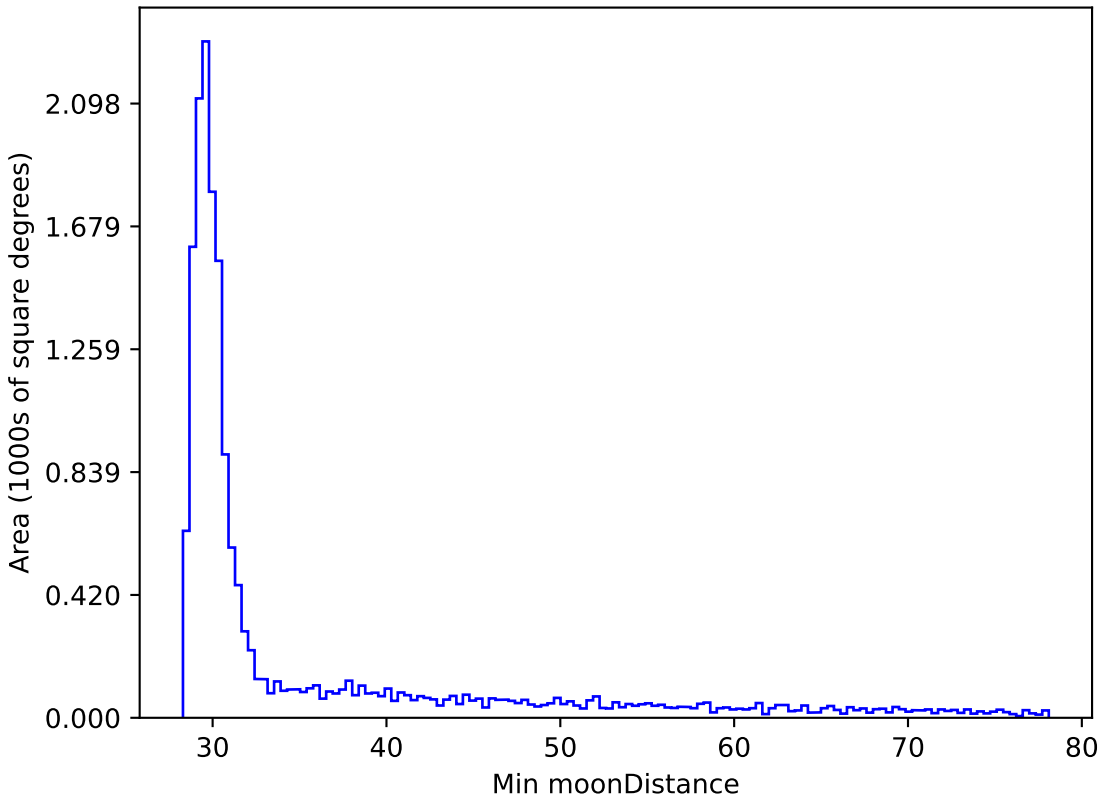
noroll_mjdp120_v3.4_10yrs WFD z band: Min moonDistance
