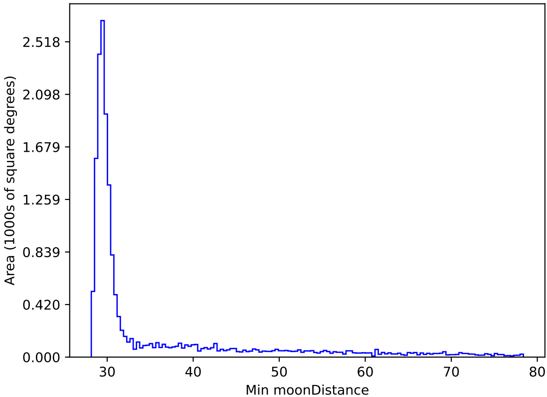
noroll_mjdp120_v3.4_10yrs WFD y band: Min moonDistance
