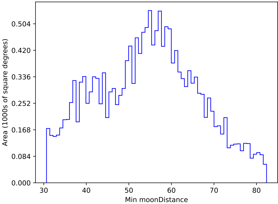
noroll_mjdp120_v3.4_10yrs WFD u band: Min moonDistance
