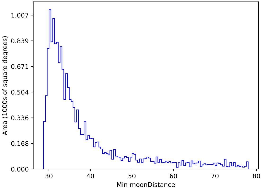
noroll_mjdp120_v3.4_10yrs WFD r band: Min moonDistance
