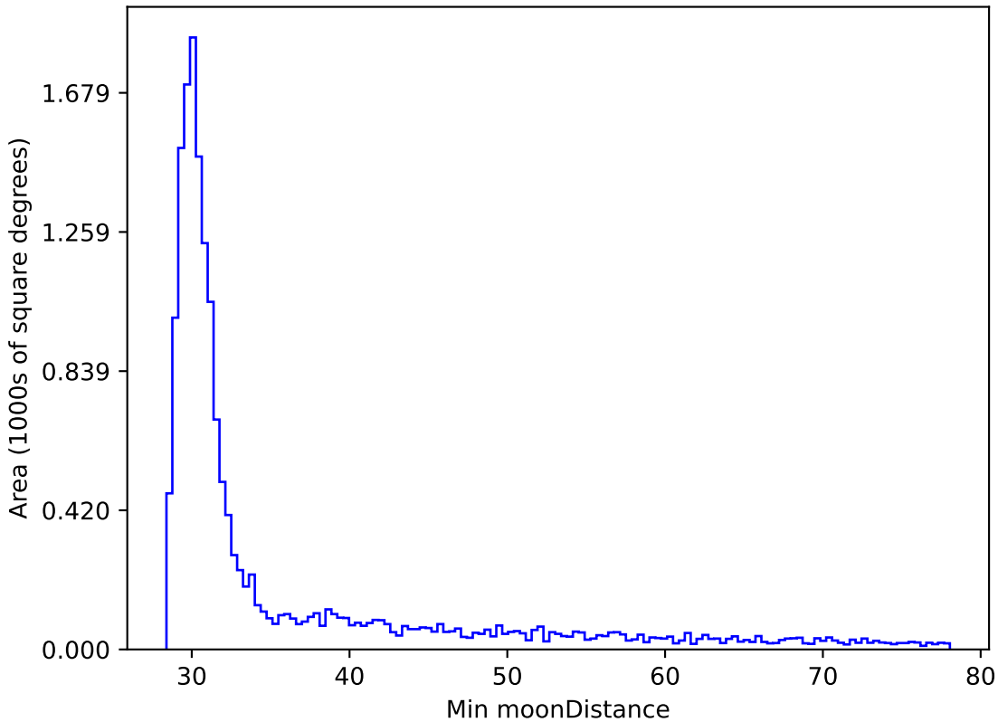
noroll_mjdp120_v3.4_10yrs WFD i band: Min moonDistance
