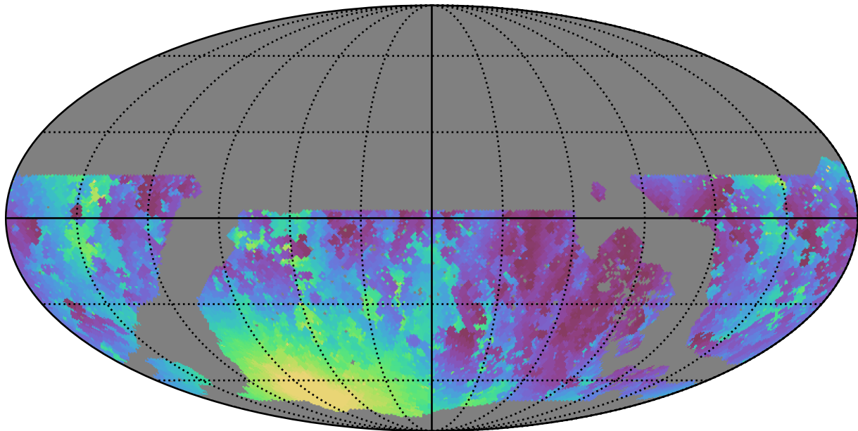
noroll_mjdp120_v3.4_10yrs WFD g band: Min moonDistance
