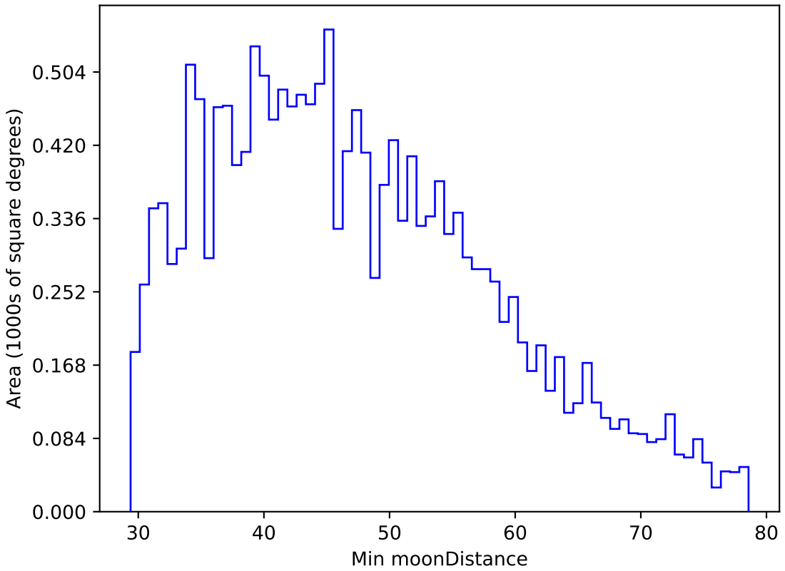
noroll_mjdp120_v3.4_10yrs WFD g band: Min moonDistance
