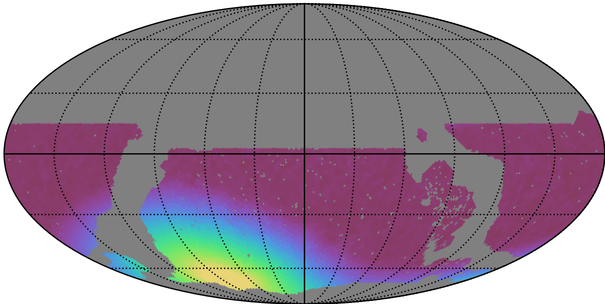
noroll_mjdp120_v3.4_10yrs WFD all bands: Min moonDistance
