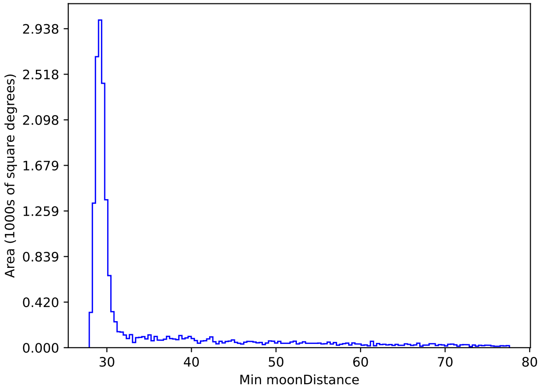
noroll_mjdp120_v3.4_10yrs WFD all bands: Min moonDistance
