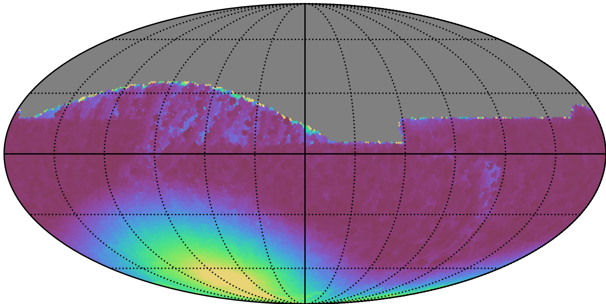
noroll_mjdp120_v3.4_10yrs All sky z band: Min moonDistance
