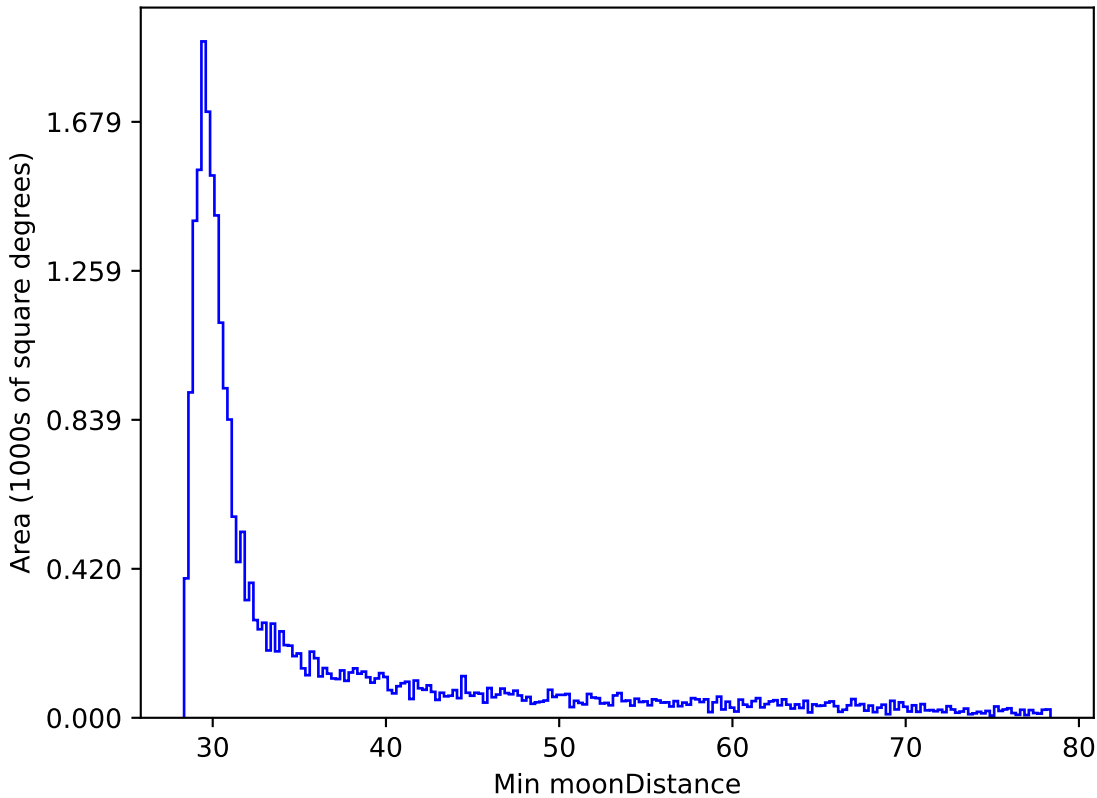
noroll_mjdp120_v3.4_10yrs All sky z band: Min moonDistance
