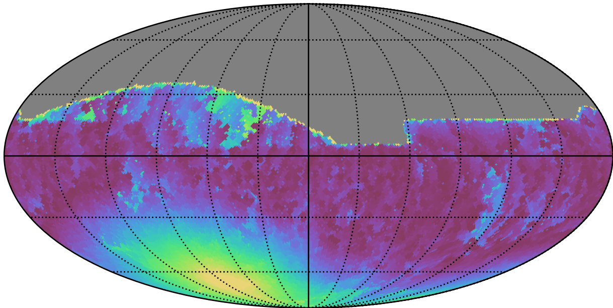
noroll_mjdp120_v3.4_10yrs All sky r band: Min moonDistance
