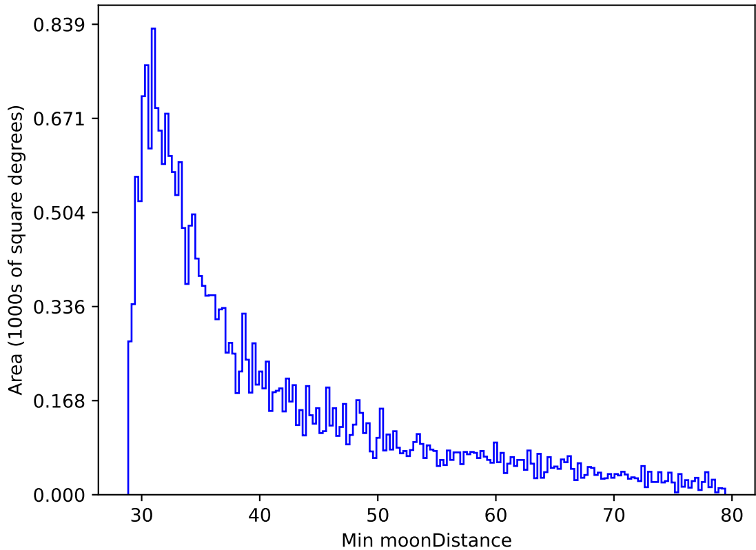
noroll_mjdp120_v3.4_10yrs All sky r band: Min moonDistance
