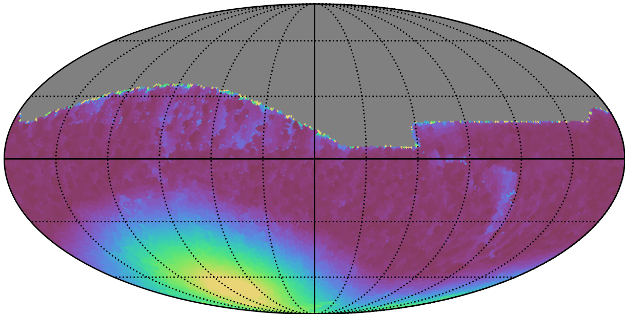
noroll_mjdp120_v3.4_10yrs All sky i band: Min moonDistance
