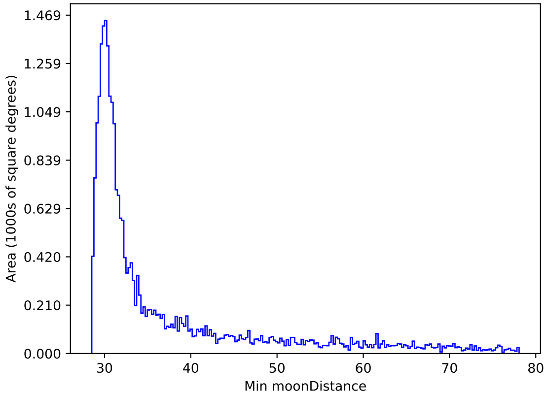
noroll_mjdp120_v3.4_10yrs All sky i band: Min moonDistance
