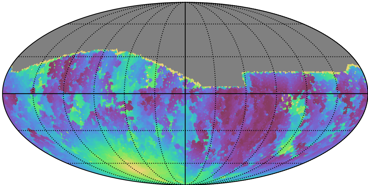
noroll_mjdp120_v3.4_10yrs All sky g band: Min moonDistance
