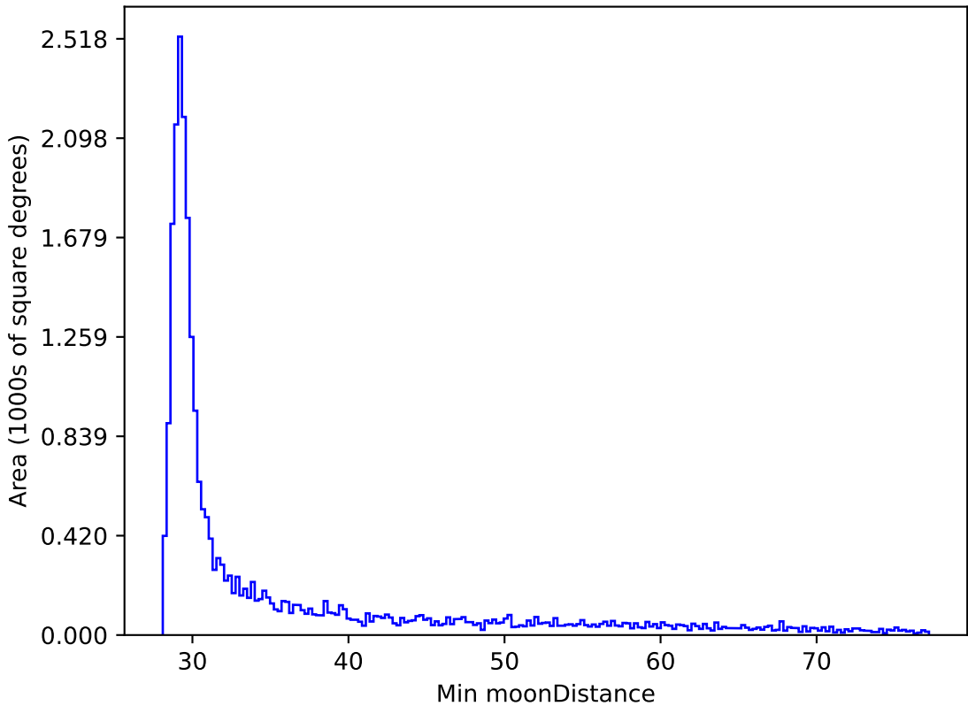
noroll_mjdp120_v3.4_10yrs All sky all bands: Min moonDistance
