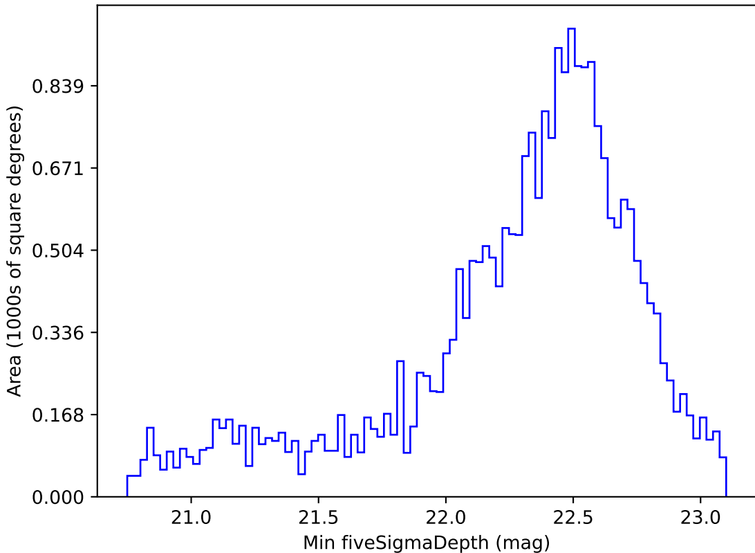
noroll_mjdp120_v3.4_10yrs Yr 1 z band: Min fiveSigmaDepth
