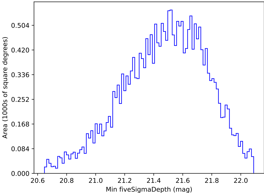
noroll_mjdp120_v3.4_10yrs Yr 1 y band: Min fiveSigmaDepth
