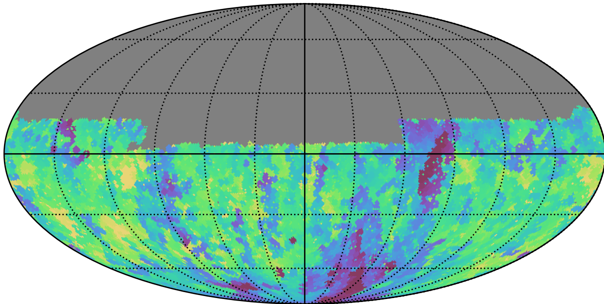
noroll_mjdp120_v3.4_10yrs Yr 1 u band: Min fiveSigmaDepth
