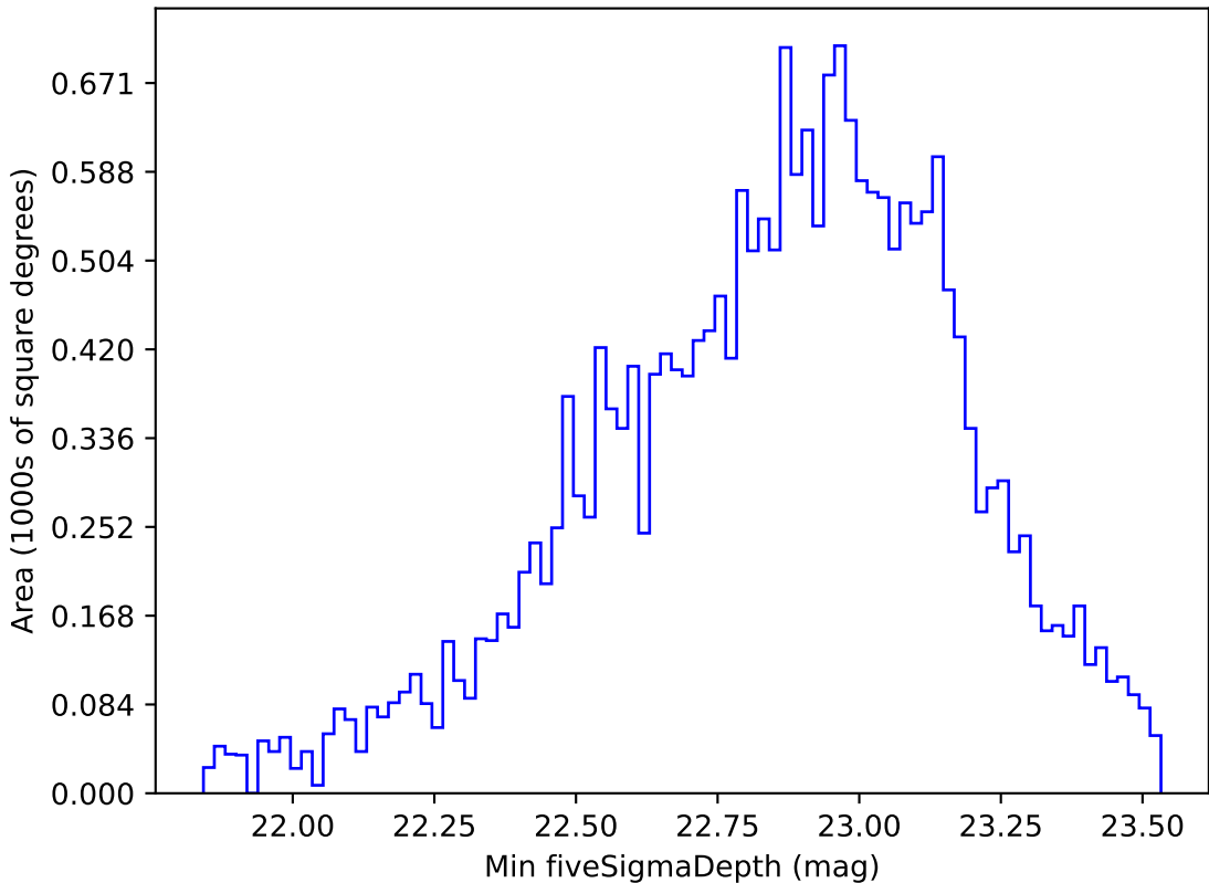
noroll_mjdp120_v3.4_10yrs Yr 1 u band: Min fiveSigmaDepth
