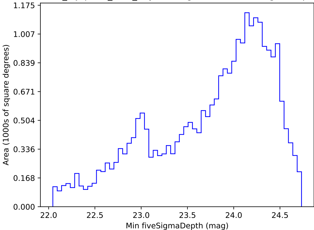
noroll_mjdp120_v3.4_10yrs Yr 1 g band: Min fiveSigmaDepth
