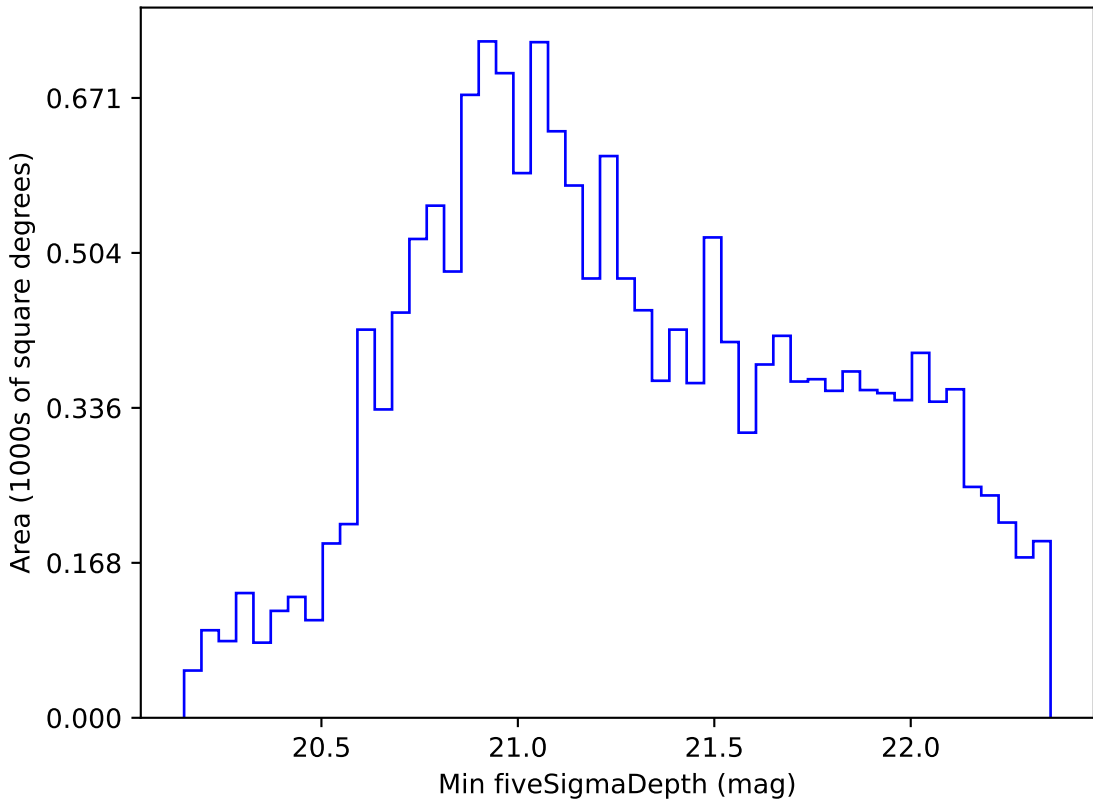
noroll_mjdp120_v3.4_10yrs WFD z band: Min fiveSigmaDepth
