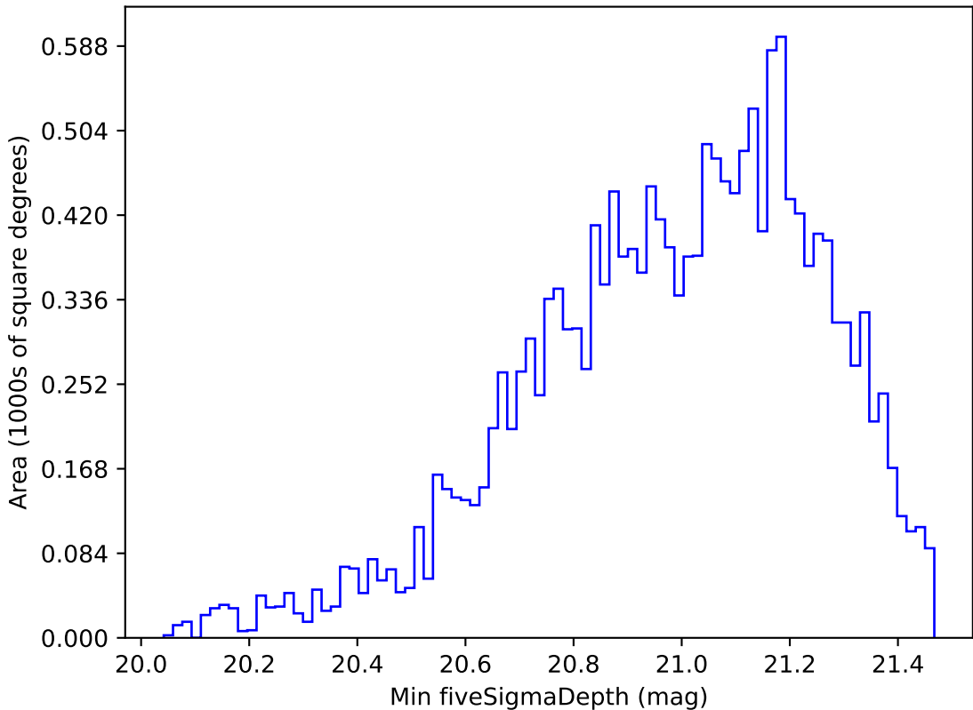
noroll_mjdp120_v3.4_10yrs WFD y band: Min fiveSigmaDepth
