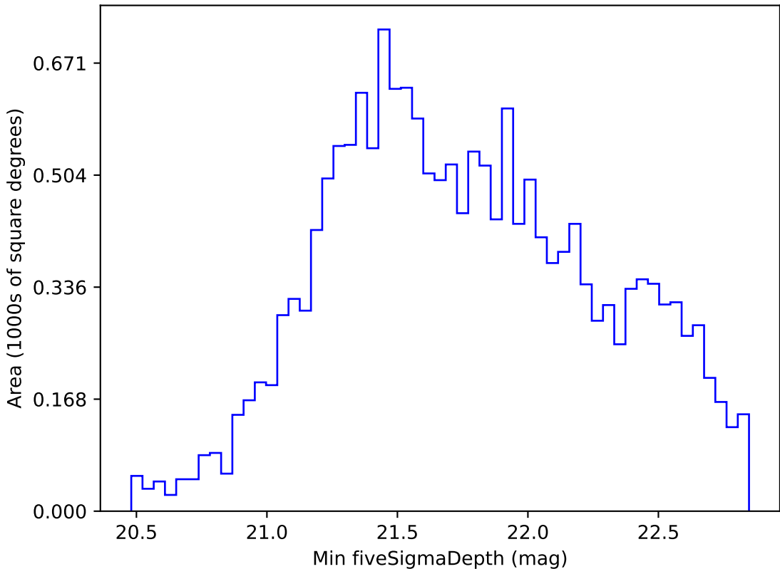
noroll_mjdp120_v3.4_10yrs WFD i band: Min fiveSigmaDepth
