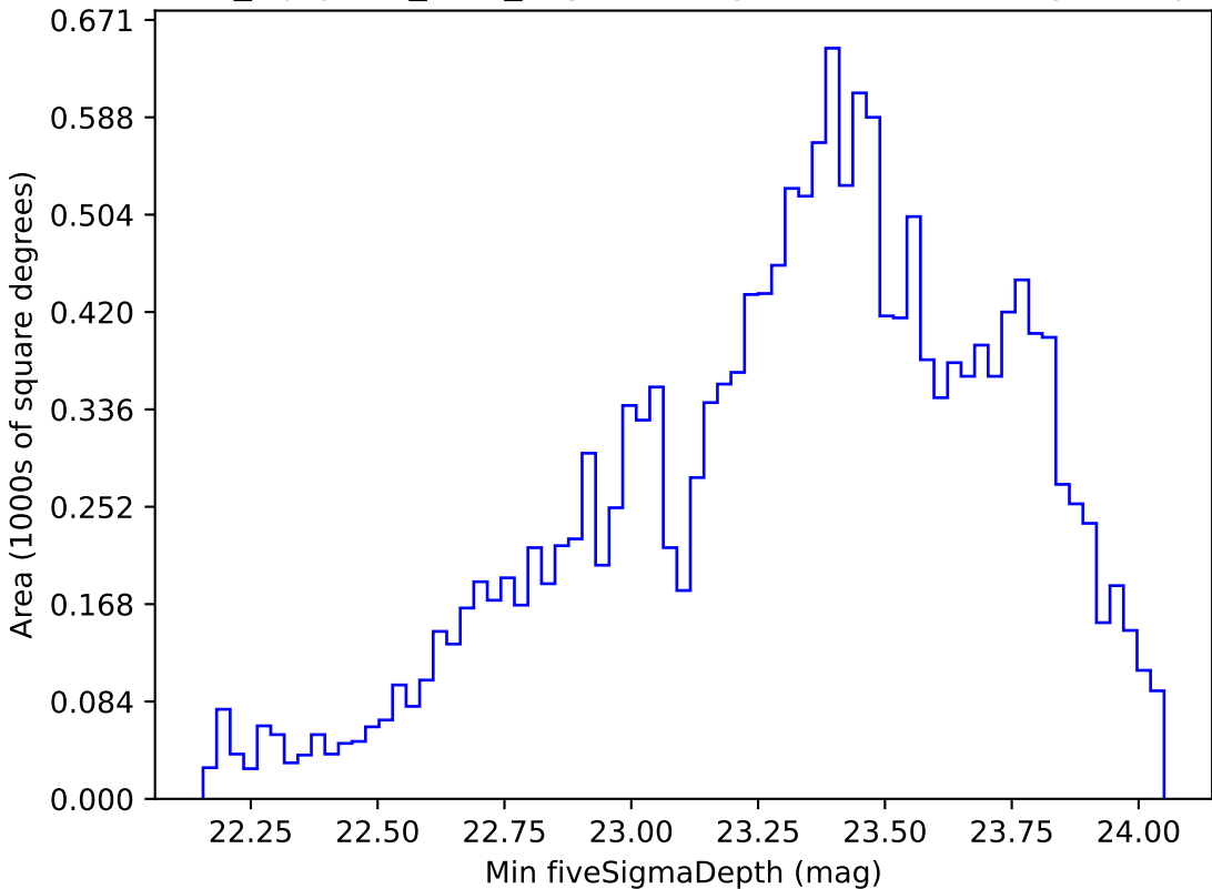
noroll_mjdp120_v3.4_10yrs WFD g band: Min fiveSigmaDepth
