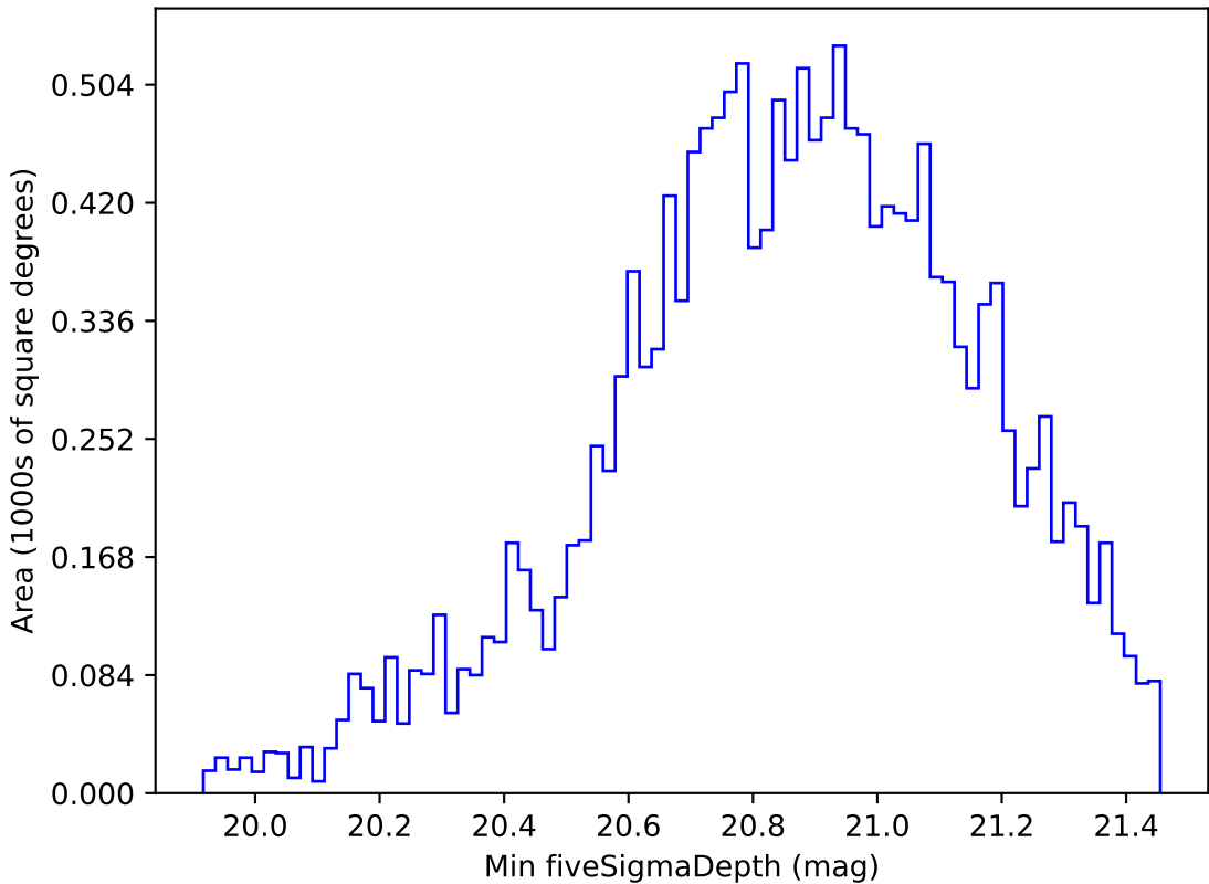
noroll_mjdp120_v3.4_10yrs WFD all bands: Min fiveSigmaDepth
