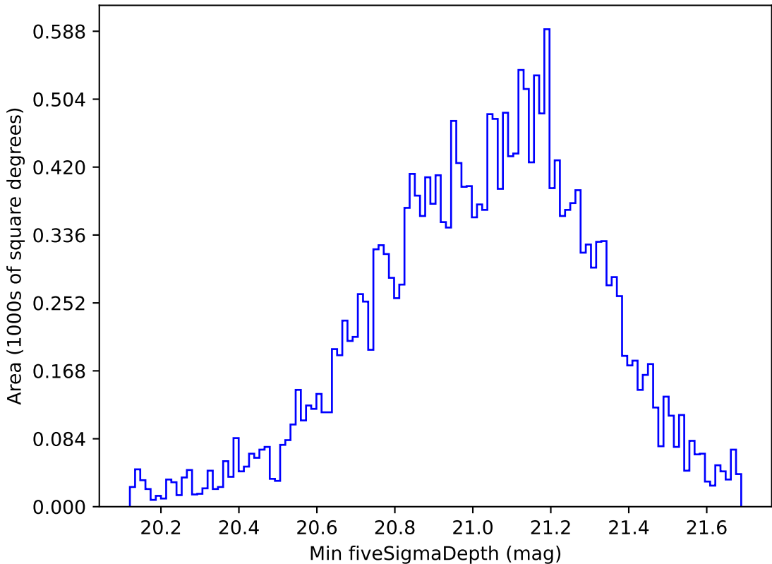
noroll_mjdp120_v3.4_10yrs All sky y band: Min fiveSigmaDepth
