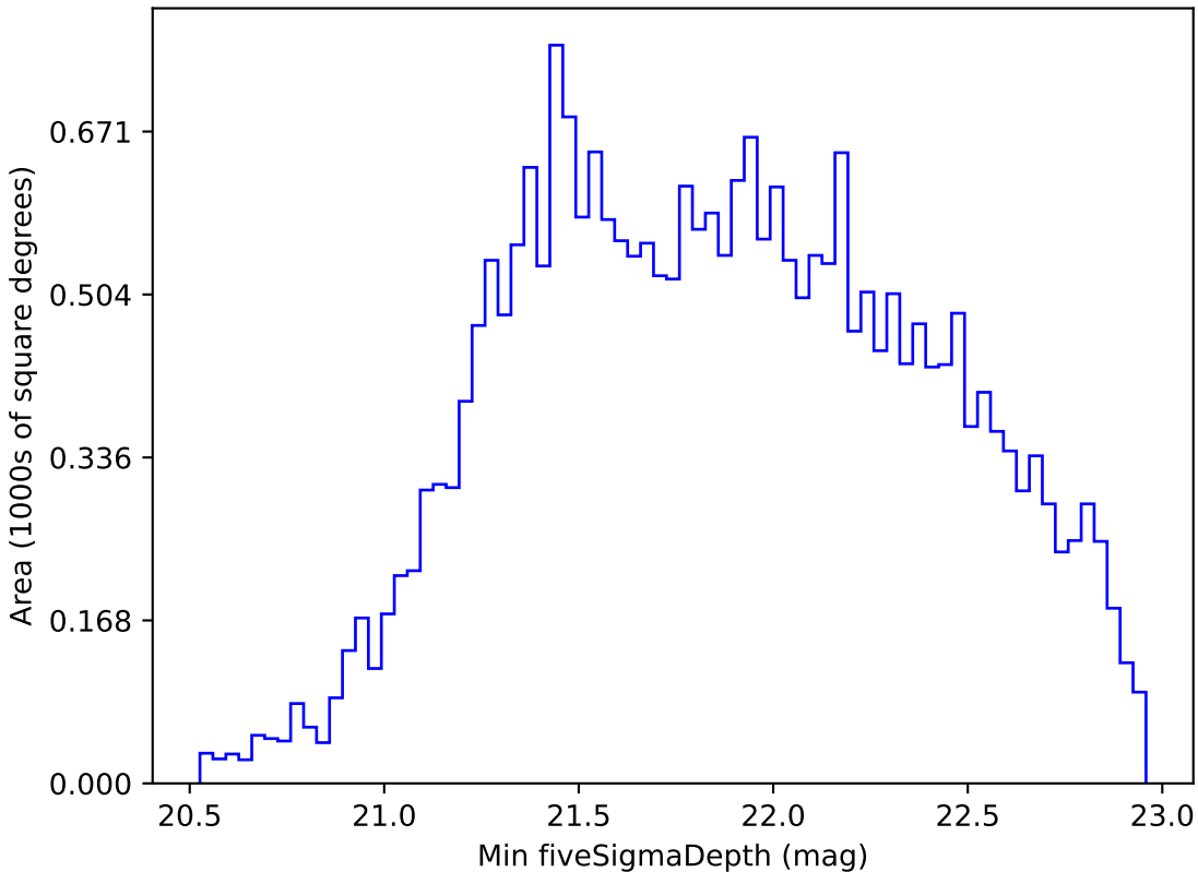
noroll_mjdp120_v3.4_10yrs All sky i band: Min fiveSigmaDepth
