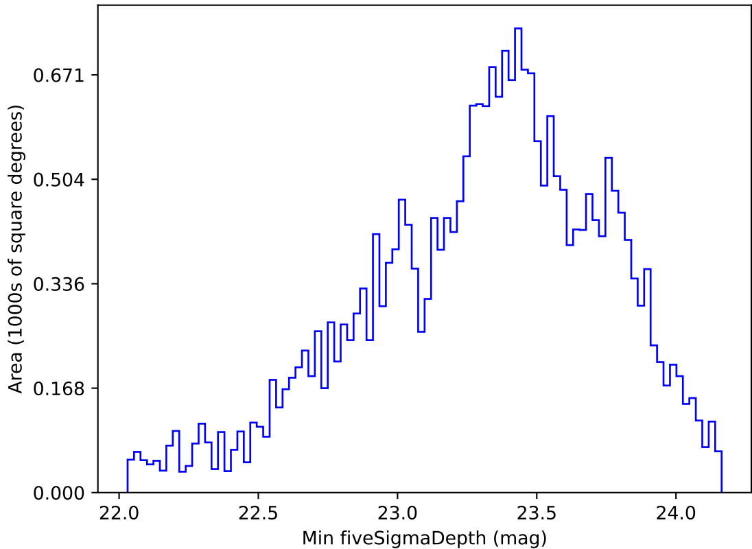
noroll_mjdp120_v3.4_10yrs All sky g band: Min fiveSigmaDepth
