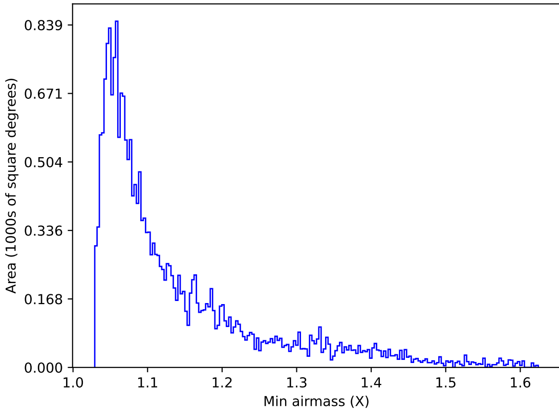
noroll_mjdp120_v3.4_10yrs Yr 1 u band: Min airmass
