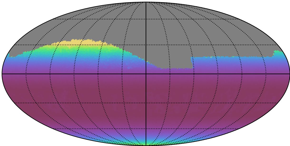
noroll_mjdp120_v3.4_10yrs Yr 1 all bands: Min airmass
